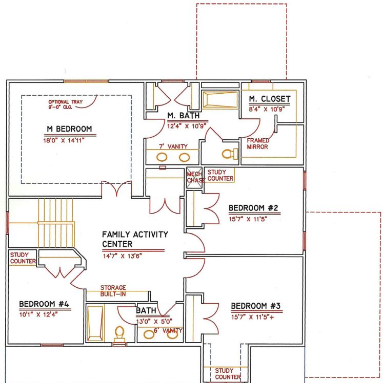
DELUXE M. BATH OPTION PARTIAL SECOND FLOOR PLAN SCALE: 1/8" = 1'-0"
