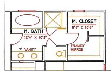
DELUXE M. BATH OPTION PARTIAL SECOND FLOOR PLAN SCALE: 1/8" = 1'-0"
