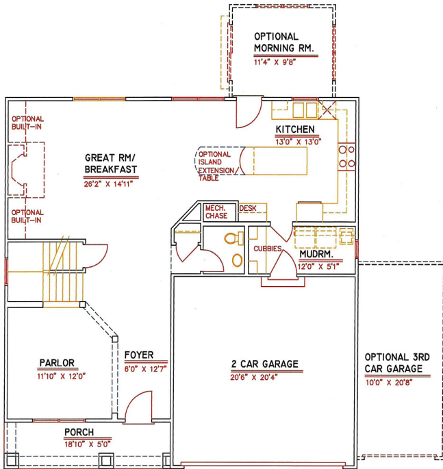
7 DAY WEEKEND - "THE NANTUCKET" FIRST FLOOR PLAN SCALE: 1/8" = 1'-0" 1073 SQ. FT.
